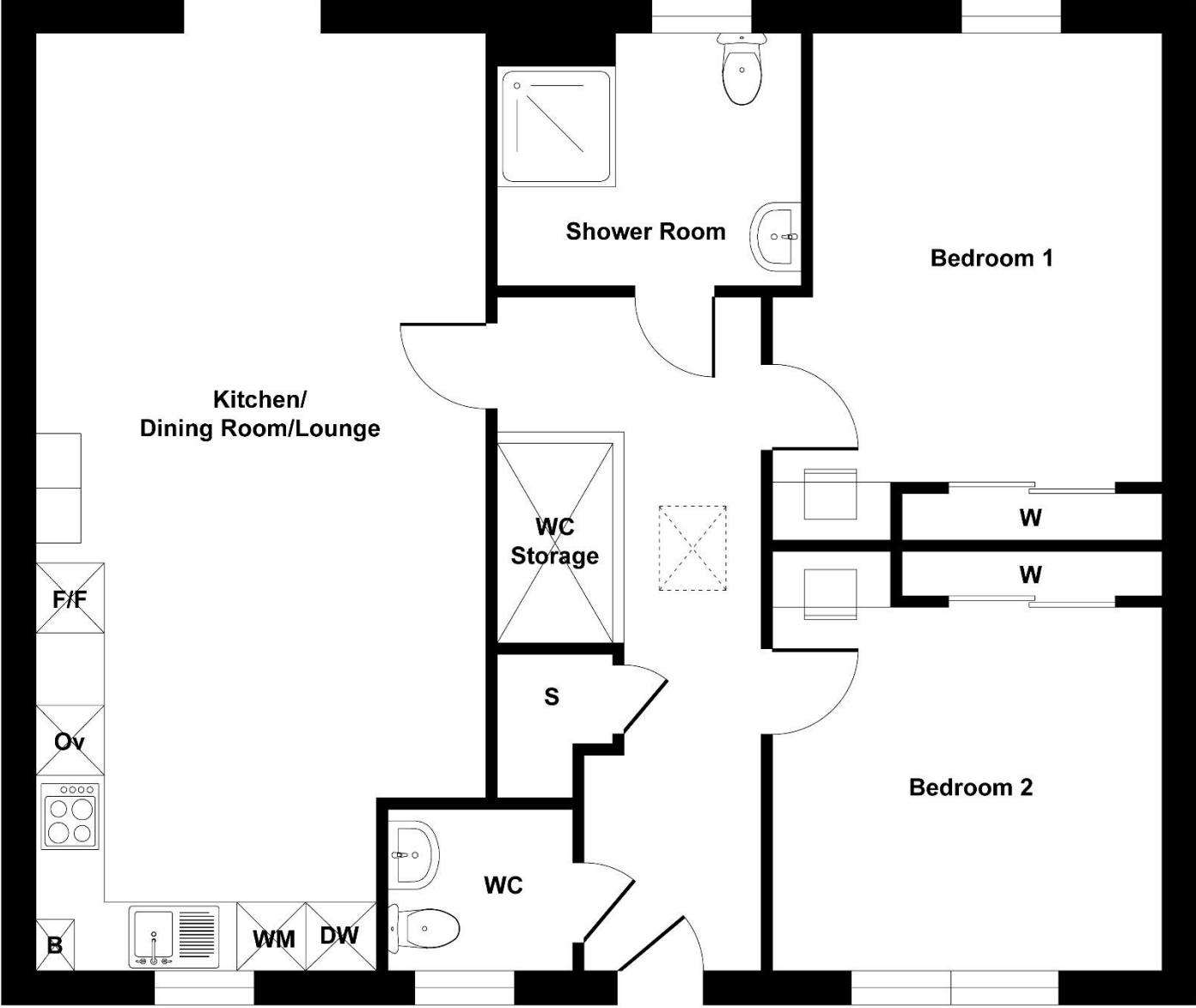
Floor Plan
