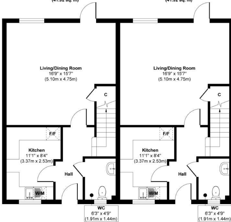
Ground Floor (Plot 296) Approximate Floor Area 451 sq. ft (41.92 sq. m)
