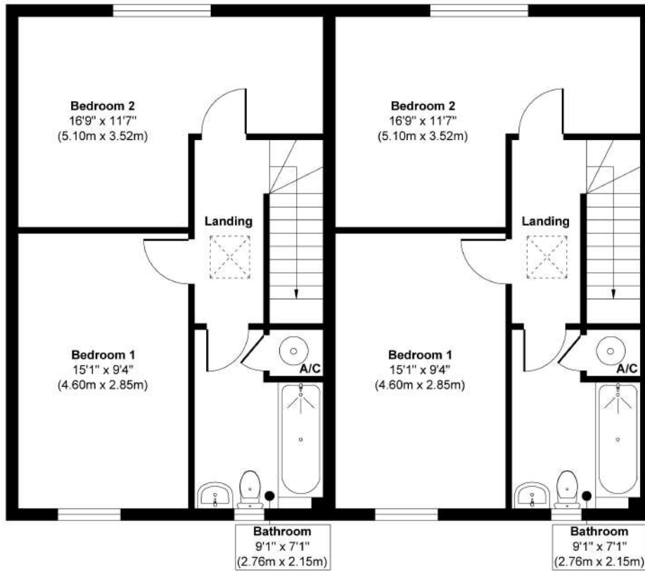
First Floor (Plot 279) Approximate Floor Area 451 sq. ft (41.92 sq. m)
